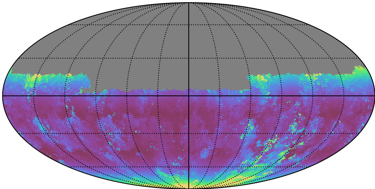
extra_ss_neo3_v3.4_10yrs Yr 1 u band: Median airmass
