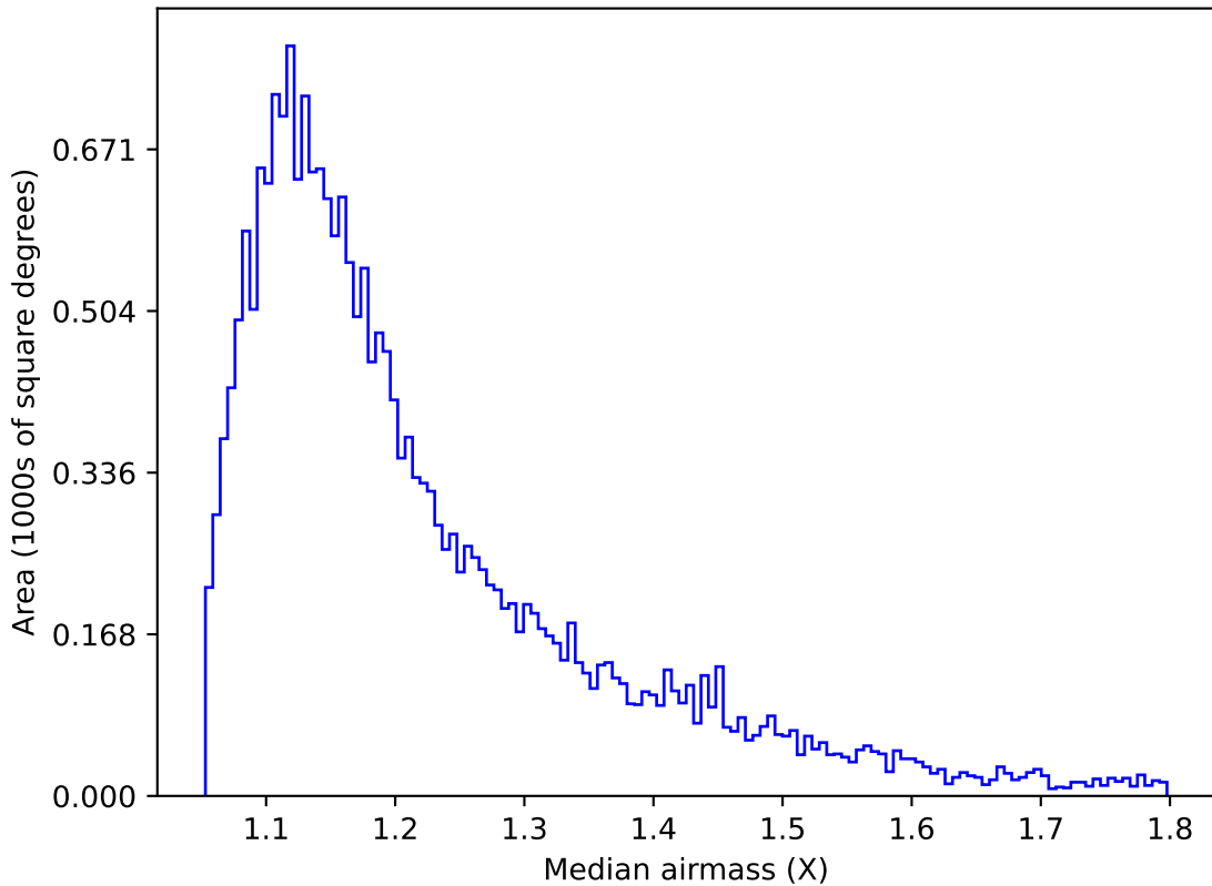
extra_ss_neo3_v3.4_10yrs Yr 1 u band: Median airmass
