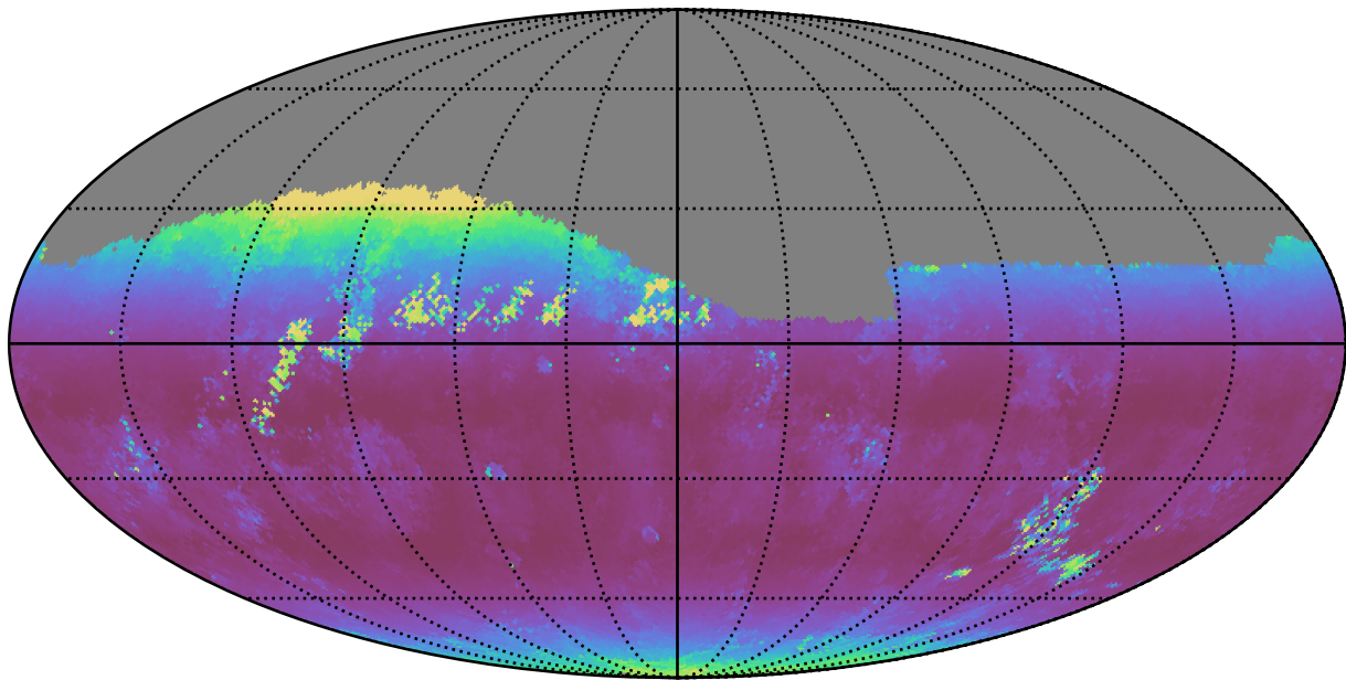
extra_ss_neo3_v3.4_10yrs Yr 1 r band: Median airmass
