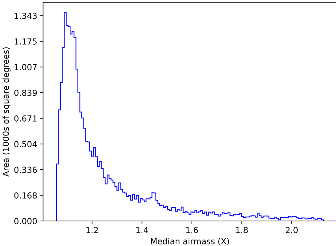
extra_ss_neo3_v3.4_10yrs Yr 1 r band: Median airmass
