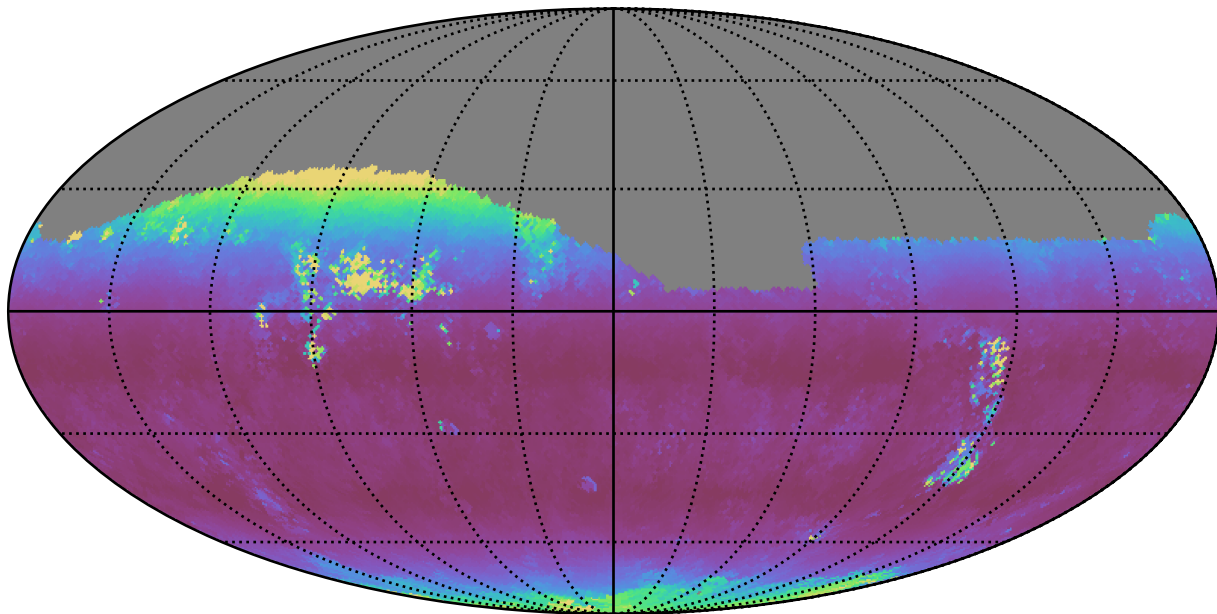
extra_ss_neo3_v3.4_10yrs Yr 1 i band: Median airmass
