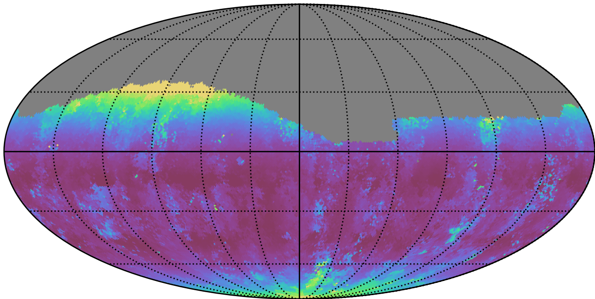
extra_ss_neo3_v3.4_10yrs Yr 1 g band: Median airmass
