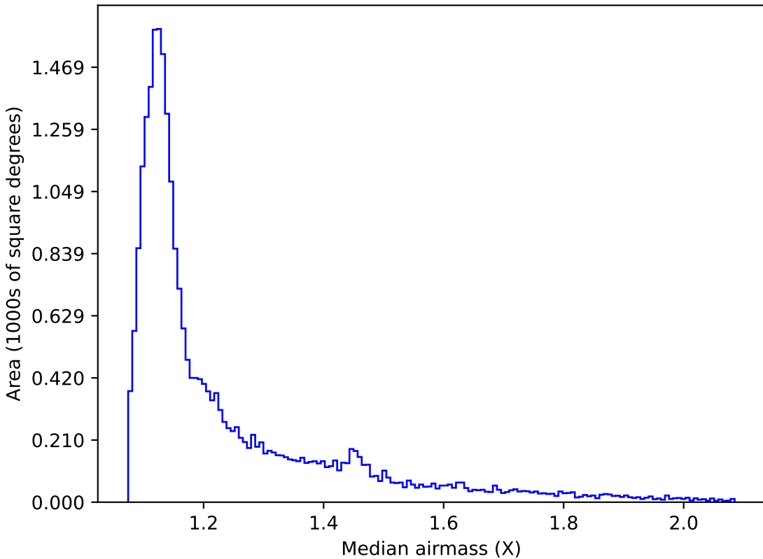
extra_ss_neo3_v3.4_10yrs Yr 1 all bands: Median airmass
