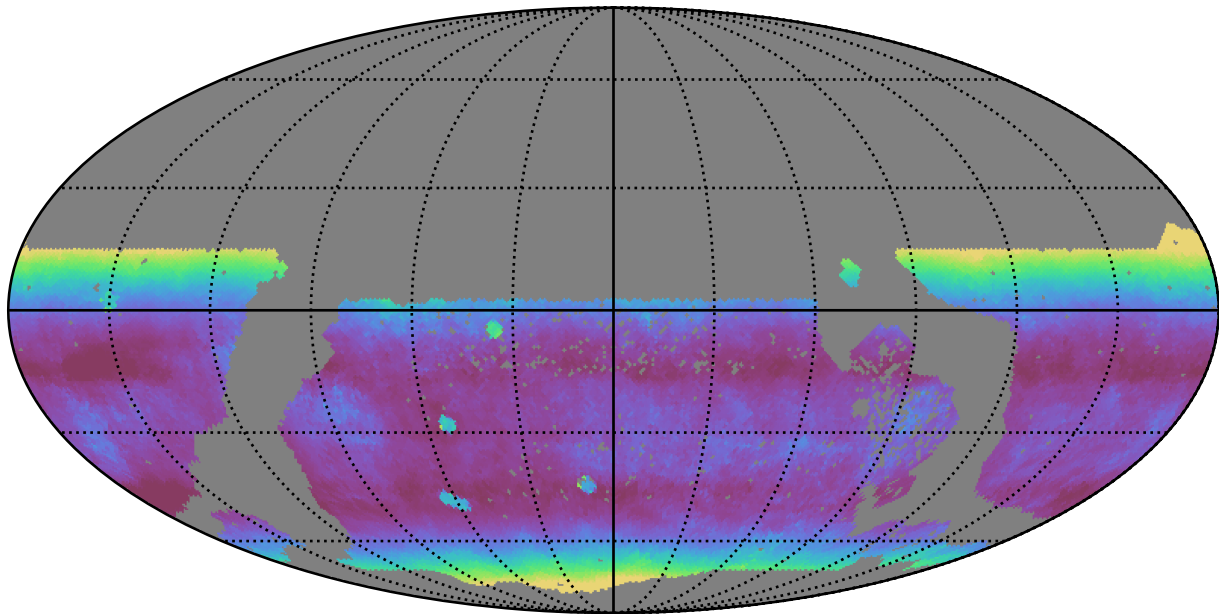
extra_ss_neo3_v3.4_10yrs WFD z band: Median airmass
