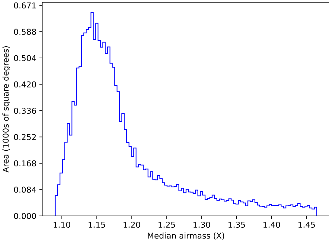
extra_ss_neo3_v3.4_10yrs WFD z band: Median airmass
