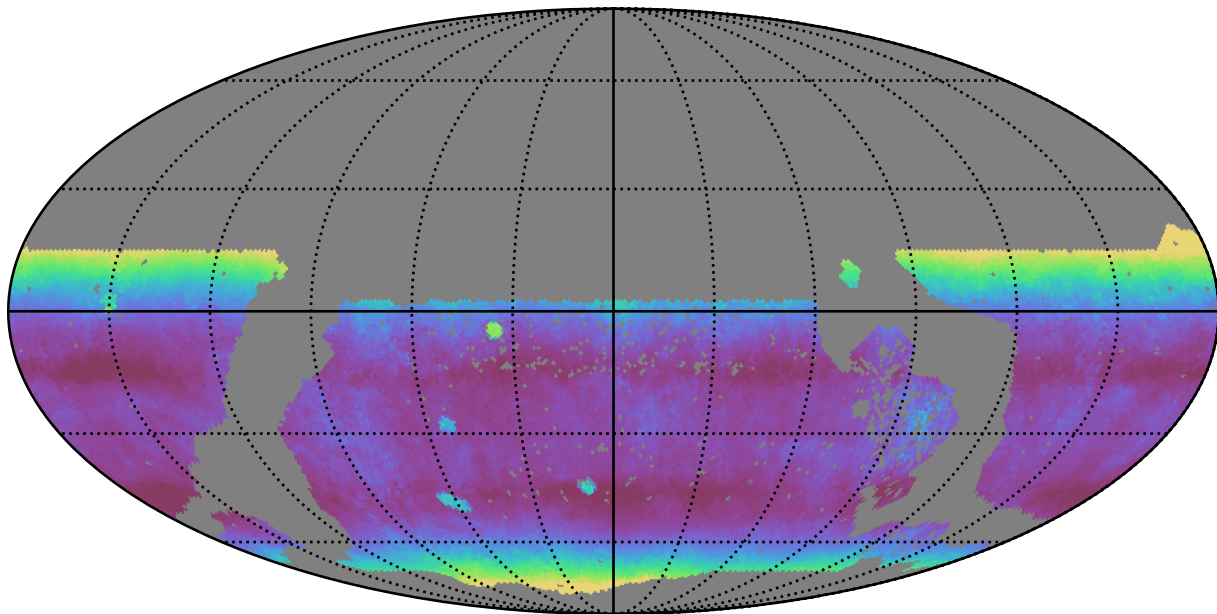
extra_ss_neo3_v3.4_10yrs WFD y band: Median airmass
