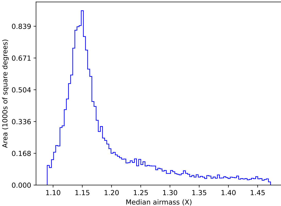
extra_ss_neo3_v3.4_10yrs WFD y band: Median airmass
