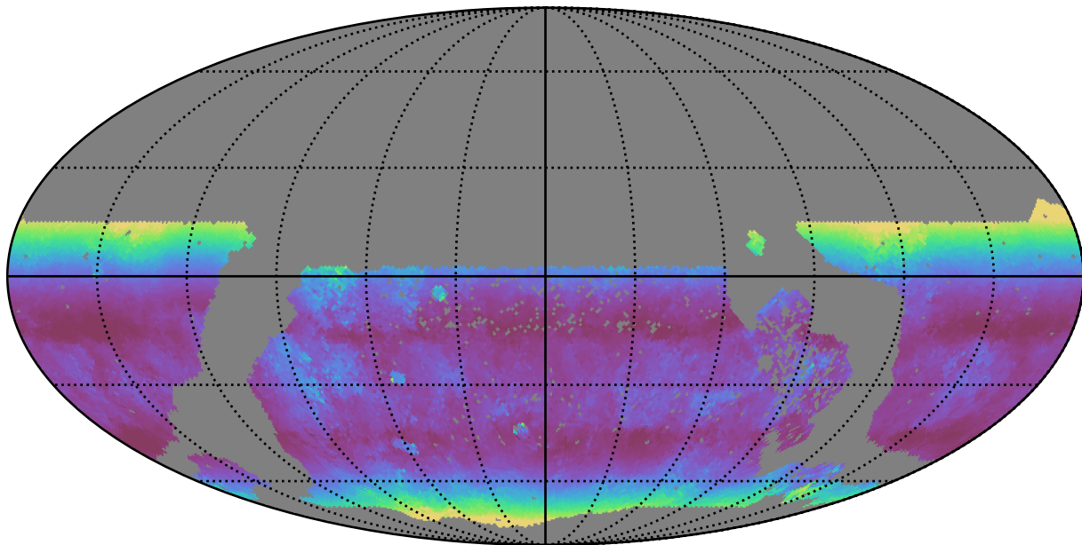
extra_ss_neo3_v3.4_10yrs WFD u band: Median airmass
