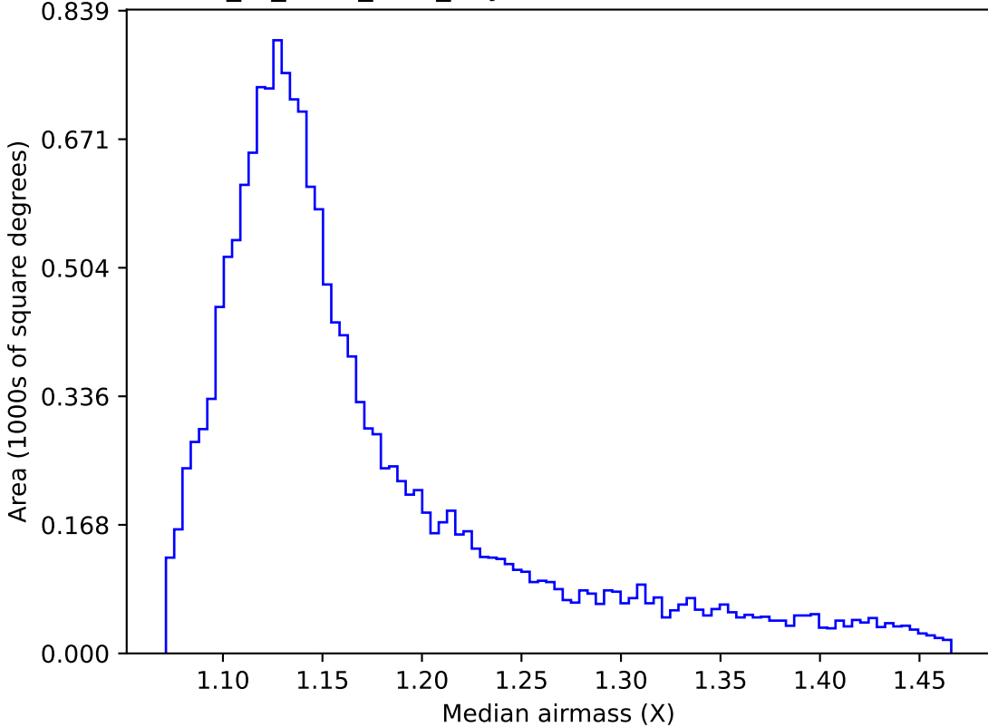
extra_ss_neo3_v3.4_10yrs WFD u band: Median airmass
