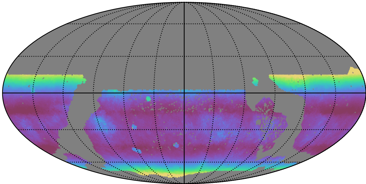
extra_ss_neo3_v3.4_10yrs WFD r band: Median airmass
