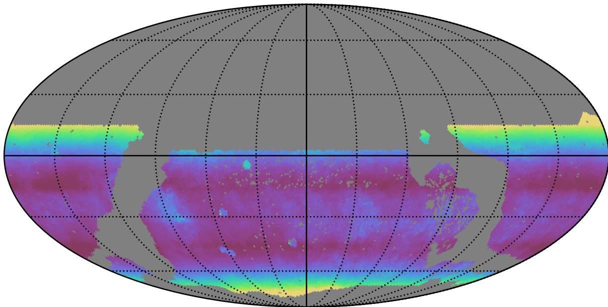
extra_ss_neo3_v3.4_10yrs WFD i band: Median airmass
