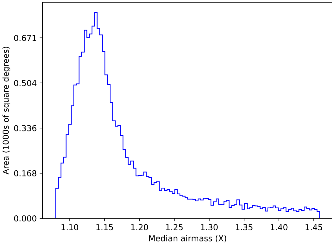
extra_ss_neo3_v3.4_10yrs WFD i band: Median airmass
