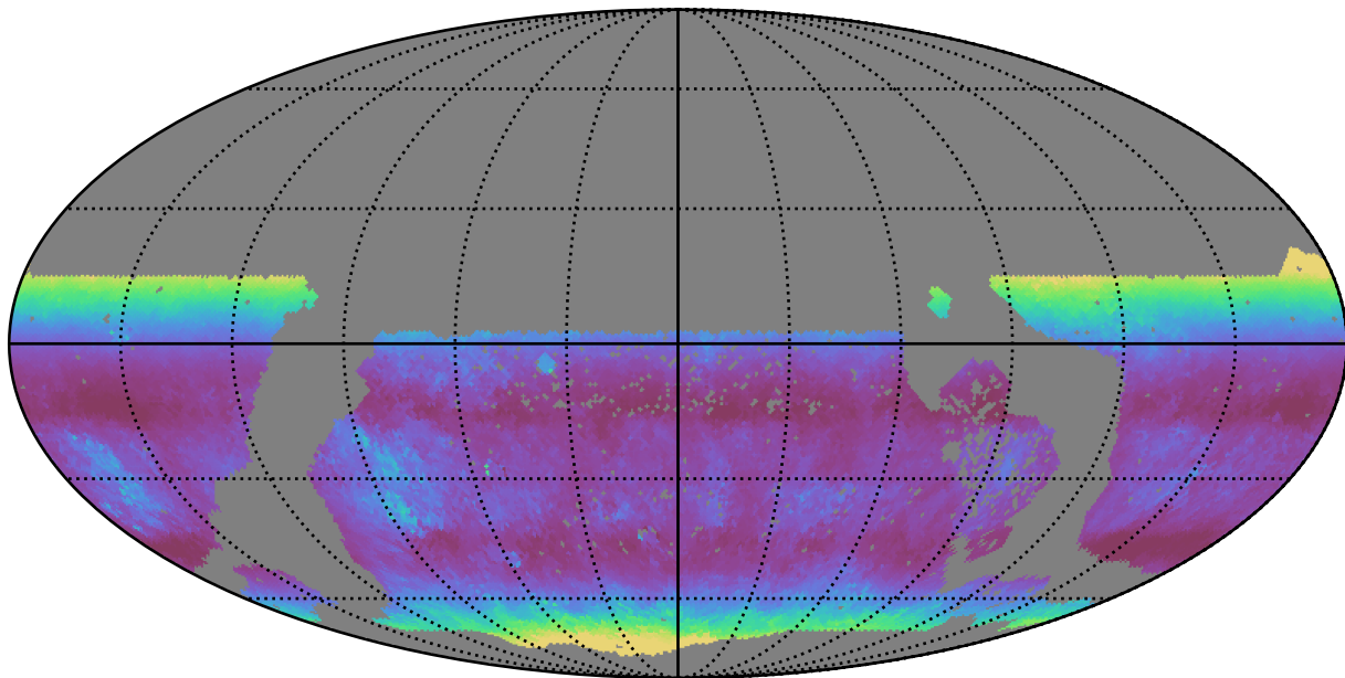
extra_ss_neo3_v3.4_10yrs WFD g band: Median airmass
