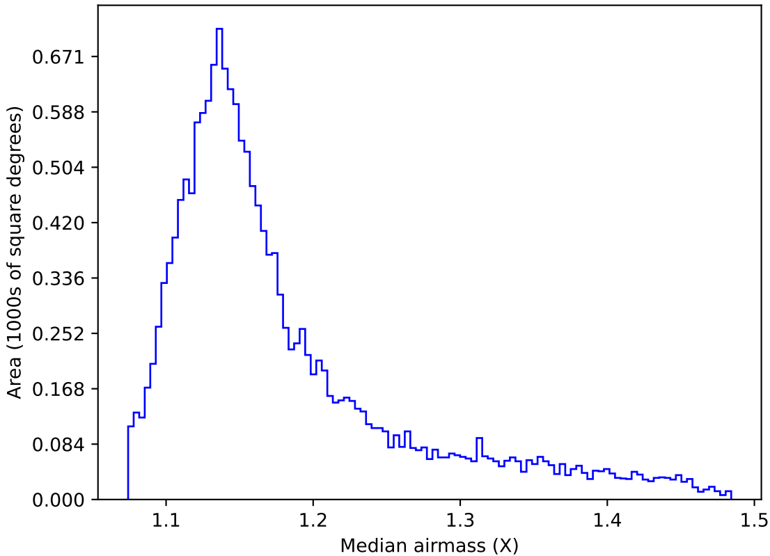
extra_ss_neo3_v3.4_10yrs WFD g band: Median airmass
