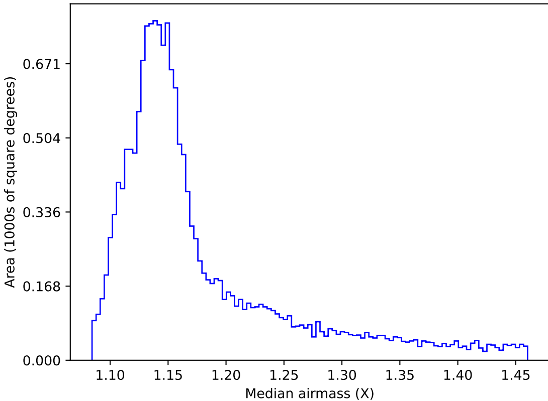
extra_ss_neo3_v3.4_10yrs WFD all bands: Median airmass
