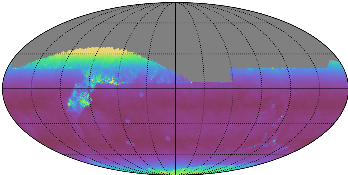
extra_ss_neo3_v3.4_10yrs All sky z band: Median airmass
