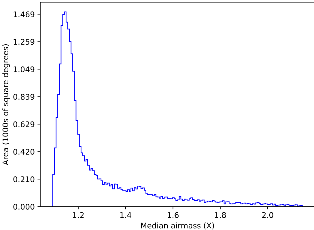
extra_ss_neo3_v3.4_10yrs All sky z band: Median airmass
