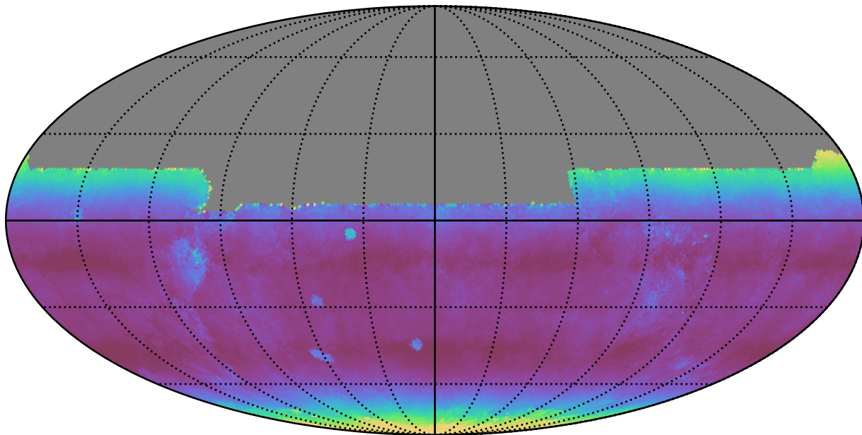
extra_ss_neo3_v3.4_10yrs All sky y band: Median airmass
