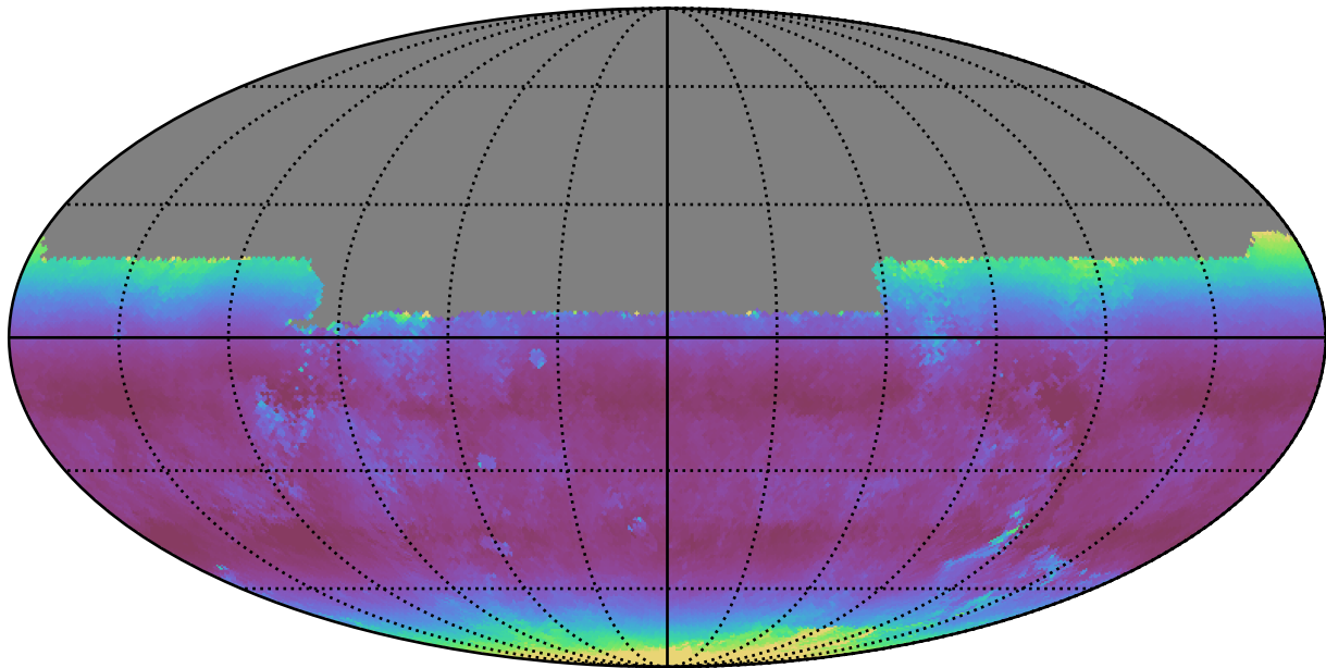
extra_ss_neo3_v3.4_10yrs All sky u band: Median airmass
