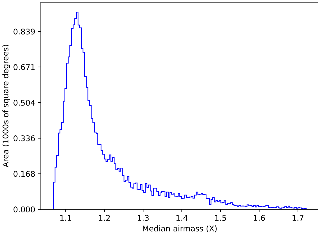
extra_ss_neo3_v3.4_10yrs All sky u band: Median airmass
