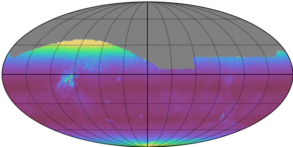
extra_ss_neo3_v3.4_10yrs All sky r band: Median airmass
