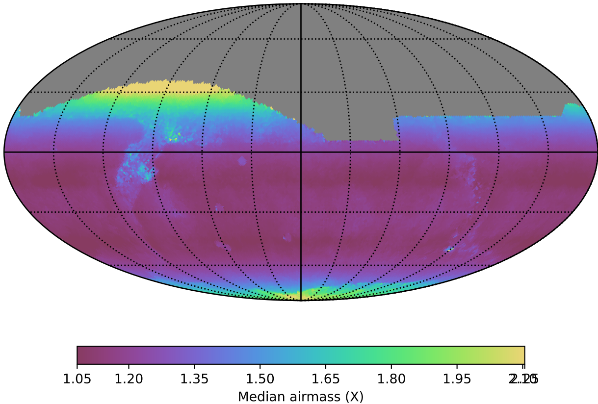
extra_ss_neo3_v3.4_10yrs All sky i band: Median airmass
