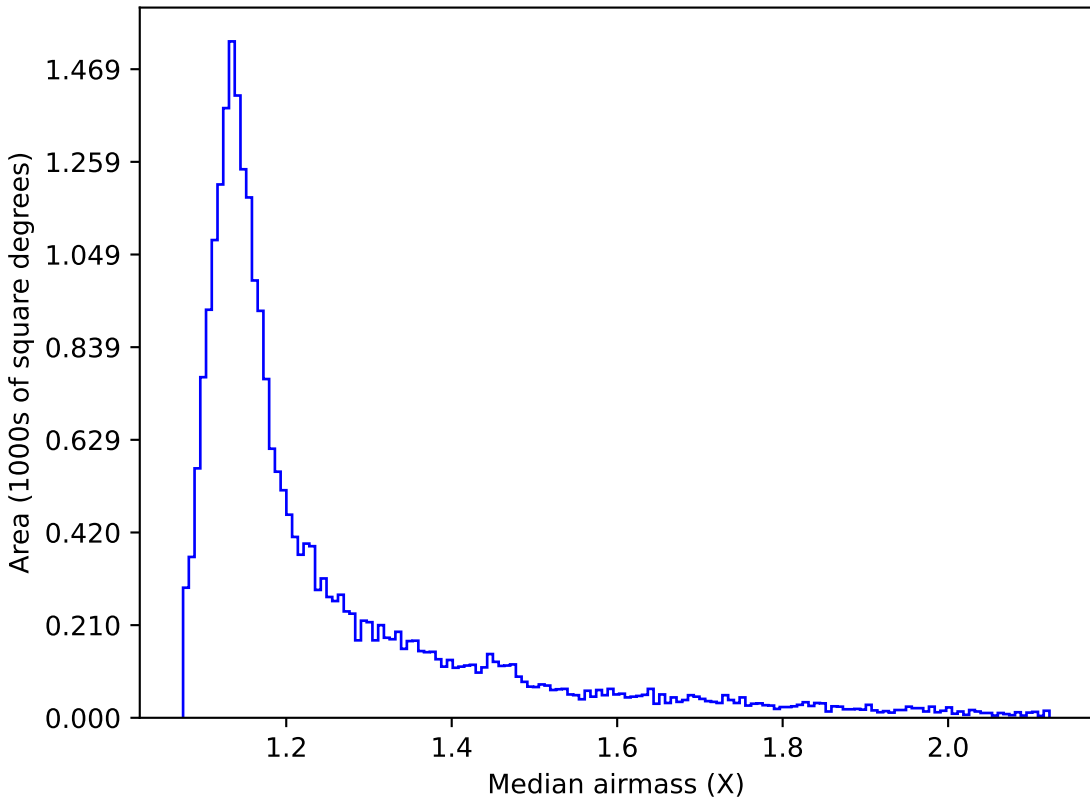
extra_ss_neo3_v3.4_10yrs All sky g band: Median airmass
