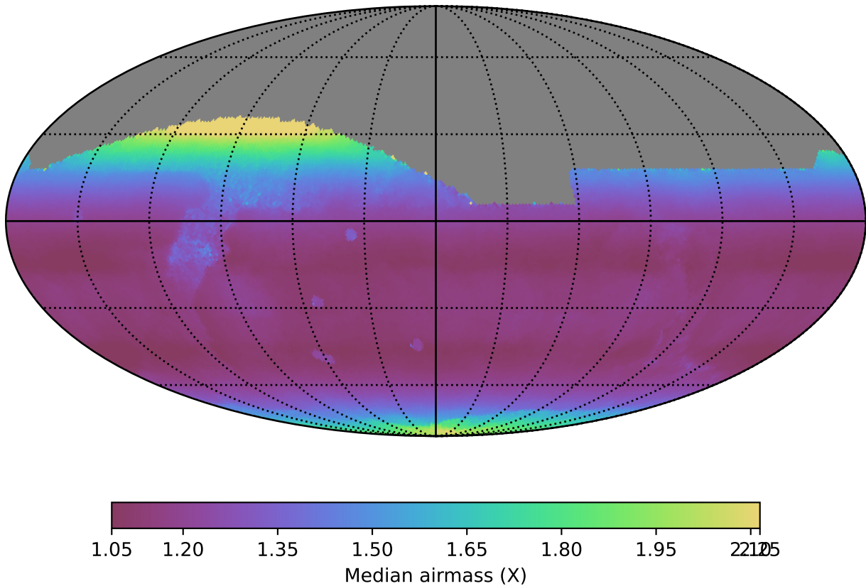
extra_ss_neo3_v3.4_10yrs All sky all bands: Median airmass
