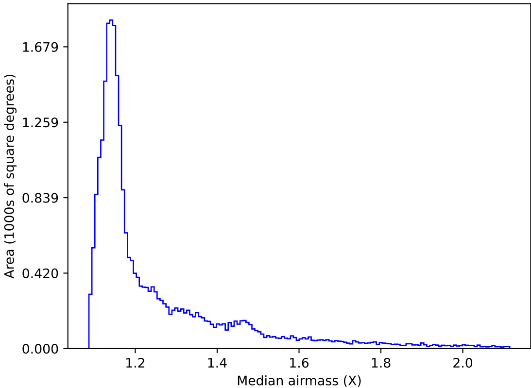
extra_ss_neo3_v3.4_10yrs All sky all bands: Median airmass
