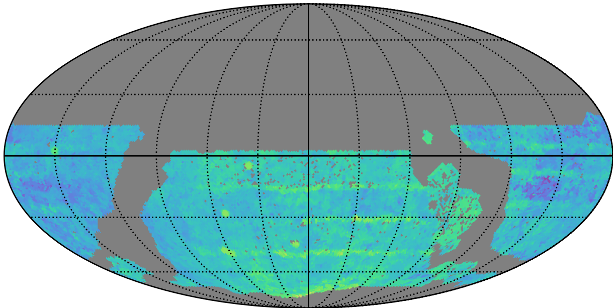
extra_ss_neo3_v3.4_10yrs WFD z band: Median Season Length
