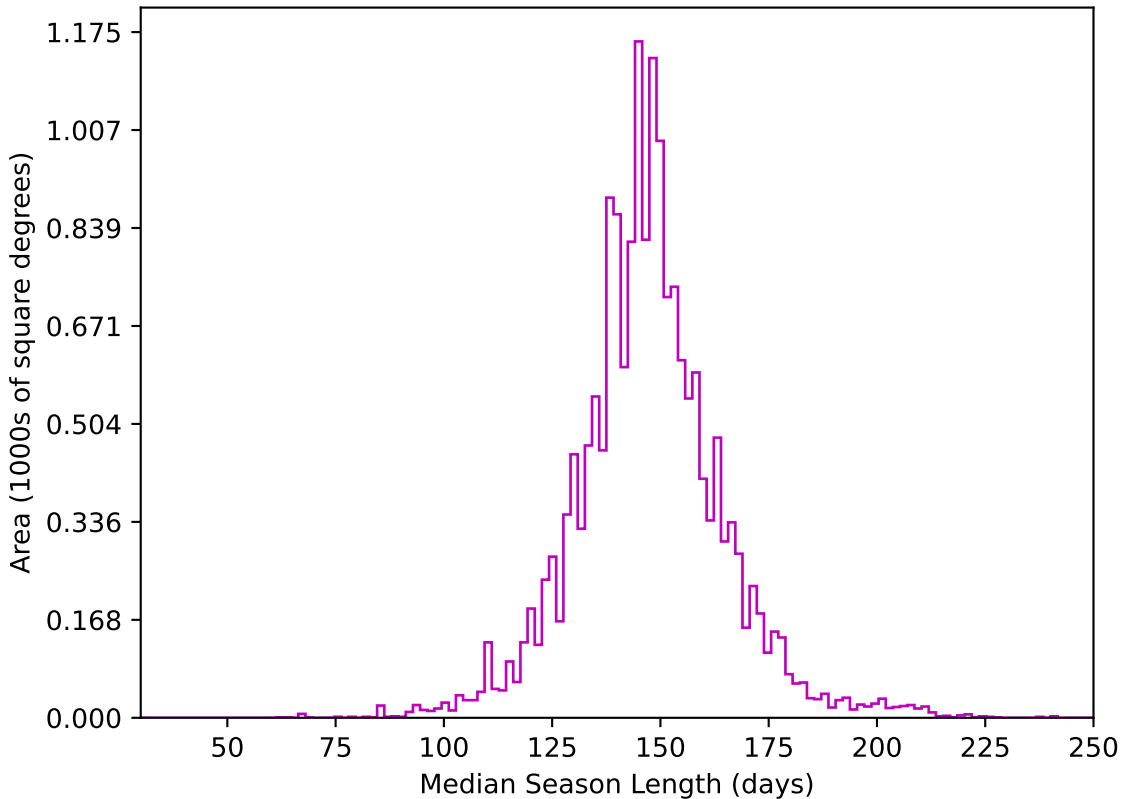
extra_ss_neo3_v3.4_10yrs WFD z band: Median Season Length
