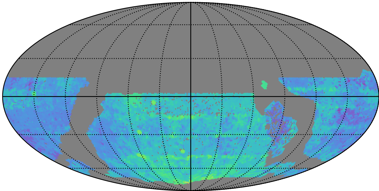
extra_ss_neo3_v3.4_10yrs WFD y band: Median Season Length
