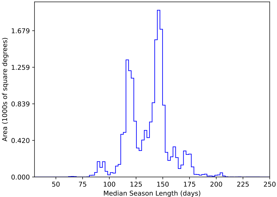
extra_ss_neo3_v3.4_10yrs WFD y band: Median Season Length
