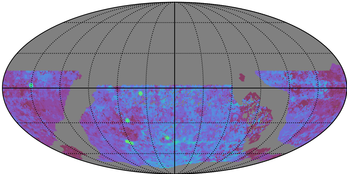
extra_ss_neo3_v3.4_10yrs WFD u band: Median Season Length
