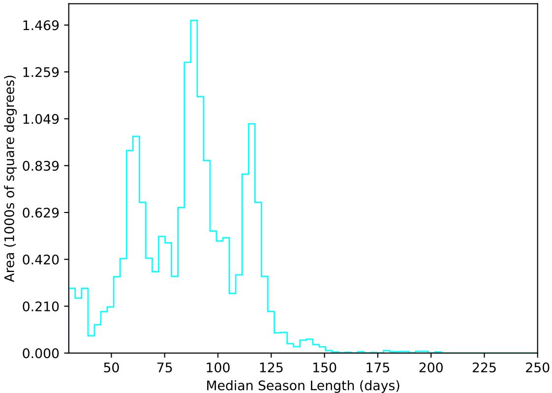
extra_ss_neo3_v3.4_10yrs WFD u band: Median Season Length
