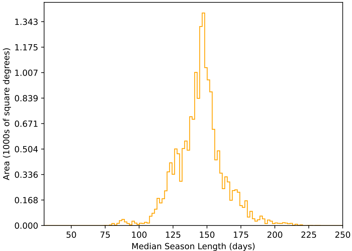
extra_ss_neo3_v3.4_10yrs WFD r band: Median Season Length
