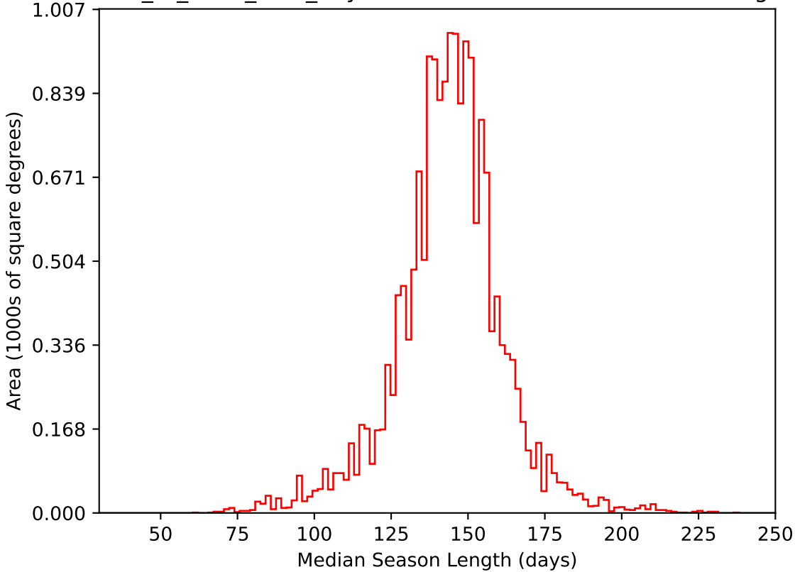
extra_ss_neo3_v3.4_10yrs WFD i band: Median Season Length
