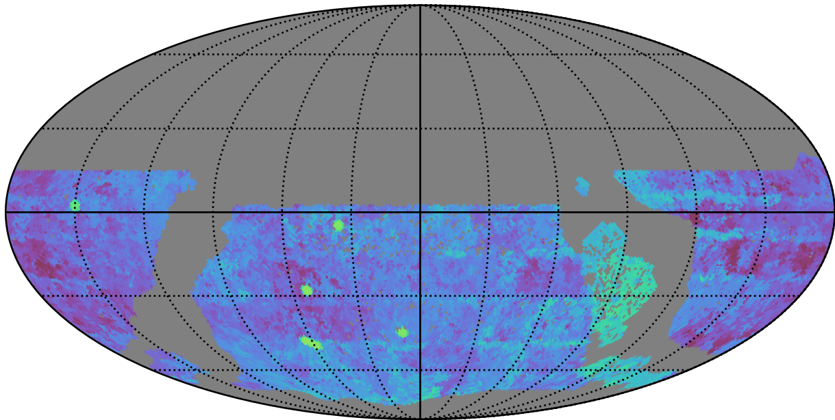
extra_ss_neo3_v3.4_10yrs WFD g band: Median Season Length
