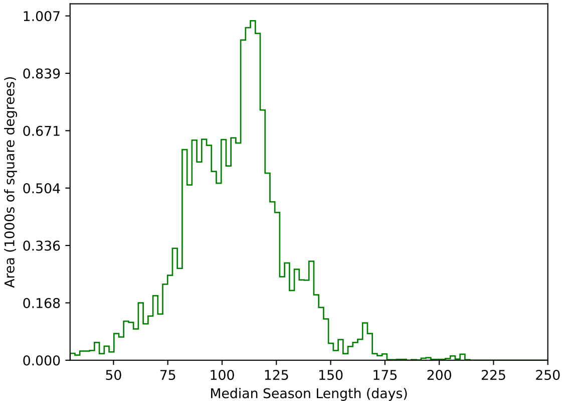
extra_ss_neo3_v3.4_10yrs WFD g band: Median Season Length
