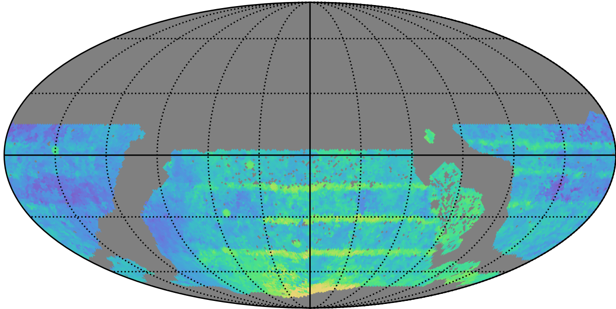
extra_ss_neo3_v3.4_10yrs WFD all bands: Median Season Length
