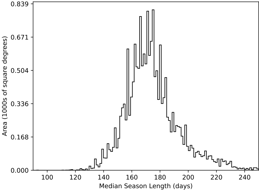
extra_ss_neo3_v3.4_10yrs WFD all bands: Median Season Length
