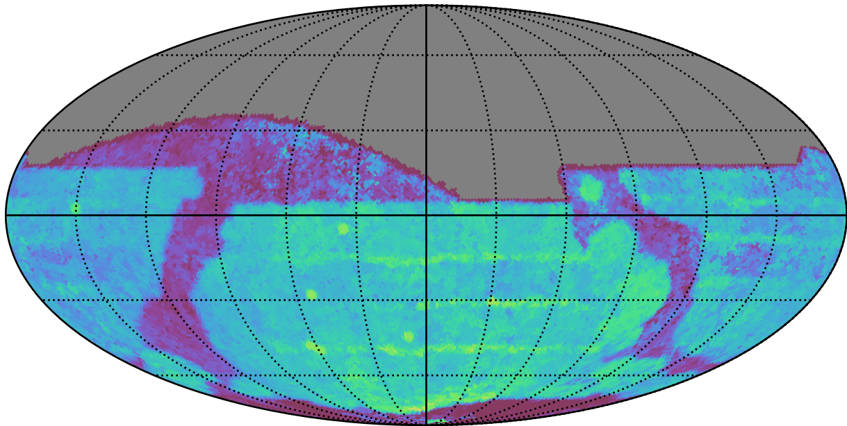
extra_ss_neo3_v3.4_10yrs All sky z band: Median Season Length
