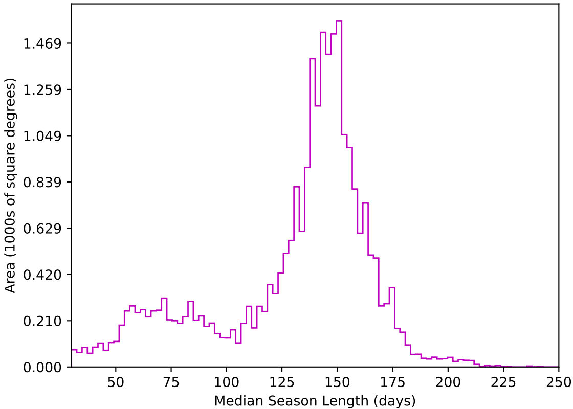
extra_ss_neo3_v3.4_10yrs All sky z band: Median Season Length
