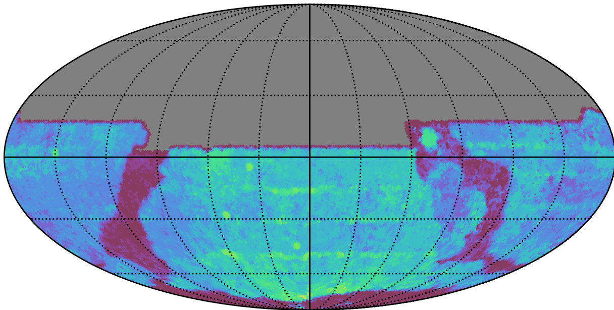
extra_ss_neo3_v3.4_10yrs All sky y band: Median Season Length
