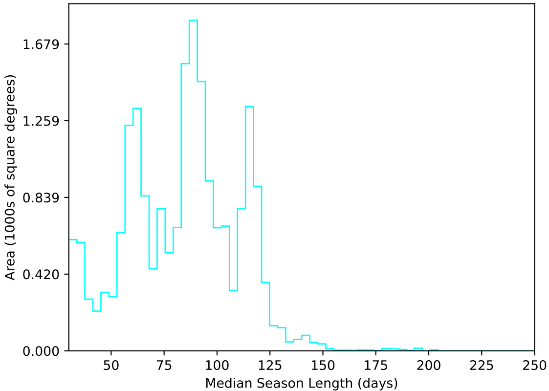
extra_ss_neo3_v3.4_10yrs All sky u band: Median Season Length
