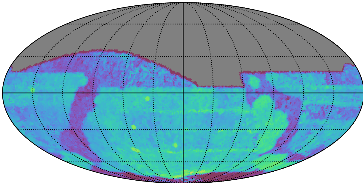
extra_ss_neo3_v3.4_10yrs All sky i band: Median Season Length
