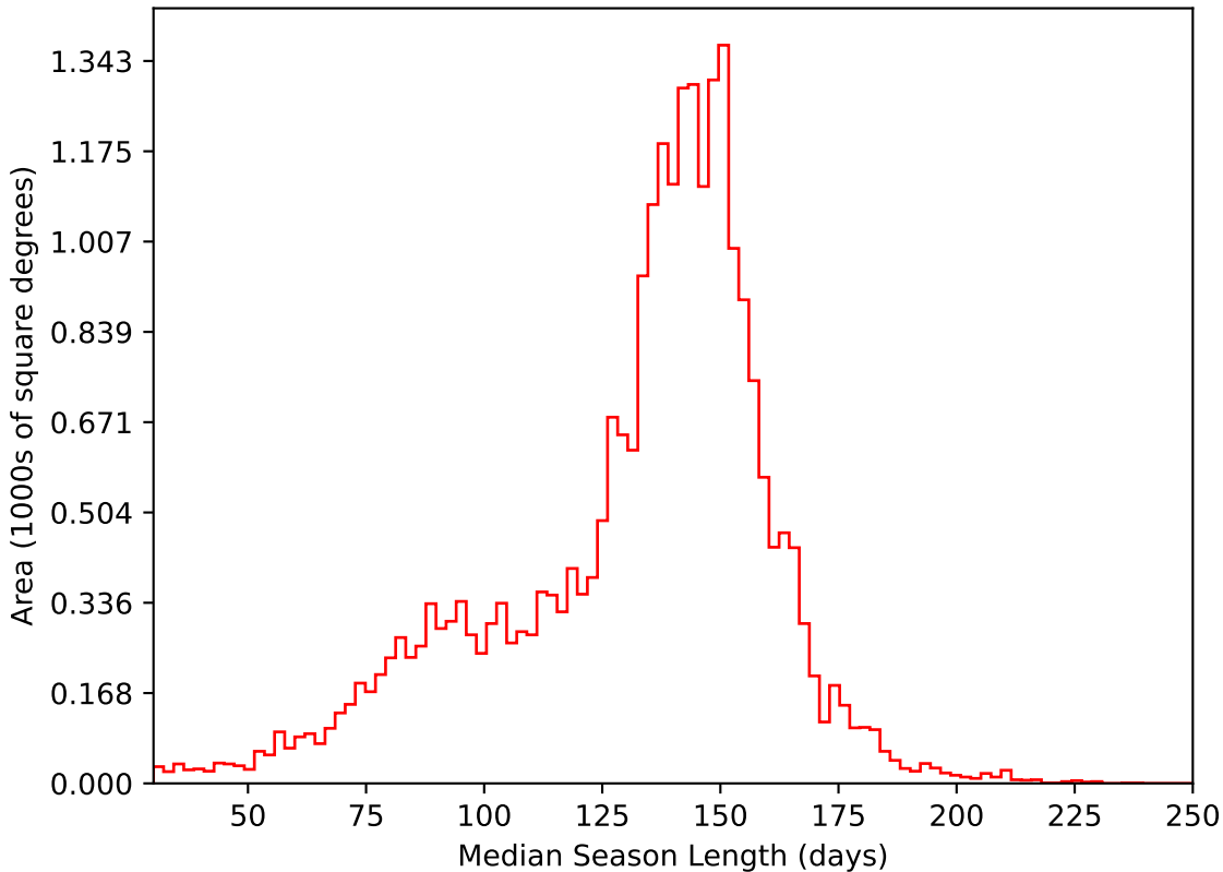
extra_ss_neo3_v3.4_10yrs All sky i band: Median Season Length
