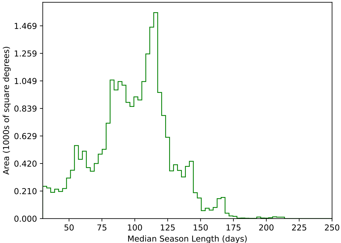
extra_ss_neo3_v3.4_10yrs All sky g band: Median Season Length
