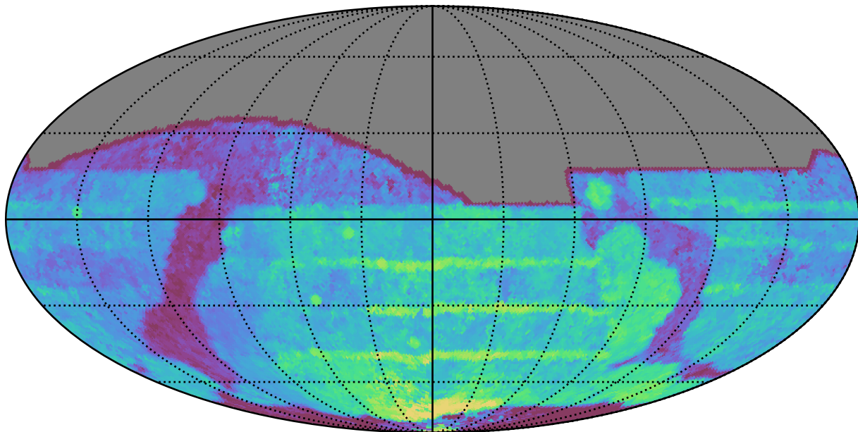
extra_ss_neo3_v3.4_10yrs All sky all bands: Median Season Length
