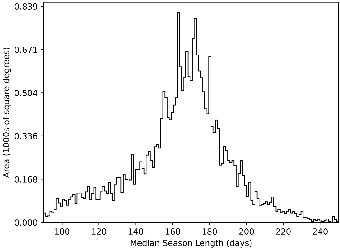
extra_ss_neo3_v3.4_10yrs All sky all bands: Median Season Length
